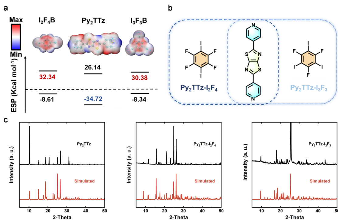
Fig. 1 (a) Calculated molecular electrostatic surface potential (ESP) visualization and extreme values for Py 2 TTz, I 2 F 4 B, and I 3 F 3 B. (b) Chemical structures of Py 2 TTz-I 2 F 4 and Py 2 TTz-I 3 F 3 . (c) XRD patterns of Py 2 TTz, Py 2 TTz-I 2 F 4 and Py 2 TTz-I 3 F 3 crystalline powders compared with simulated XRD patterns.
