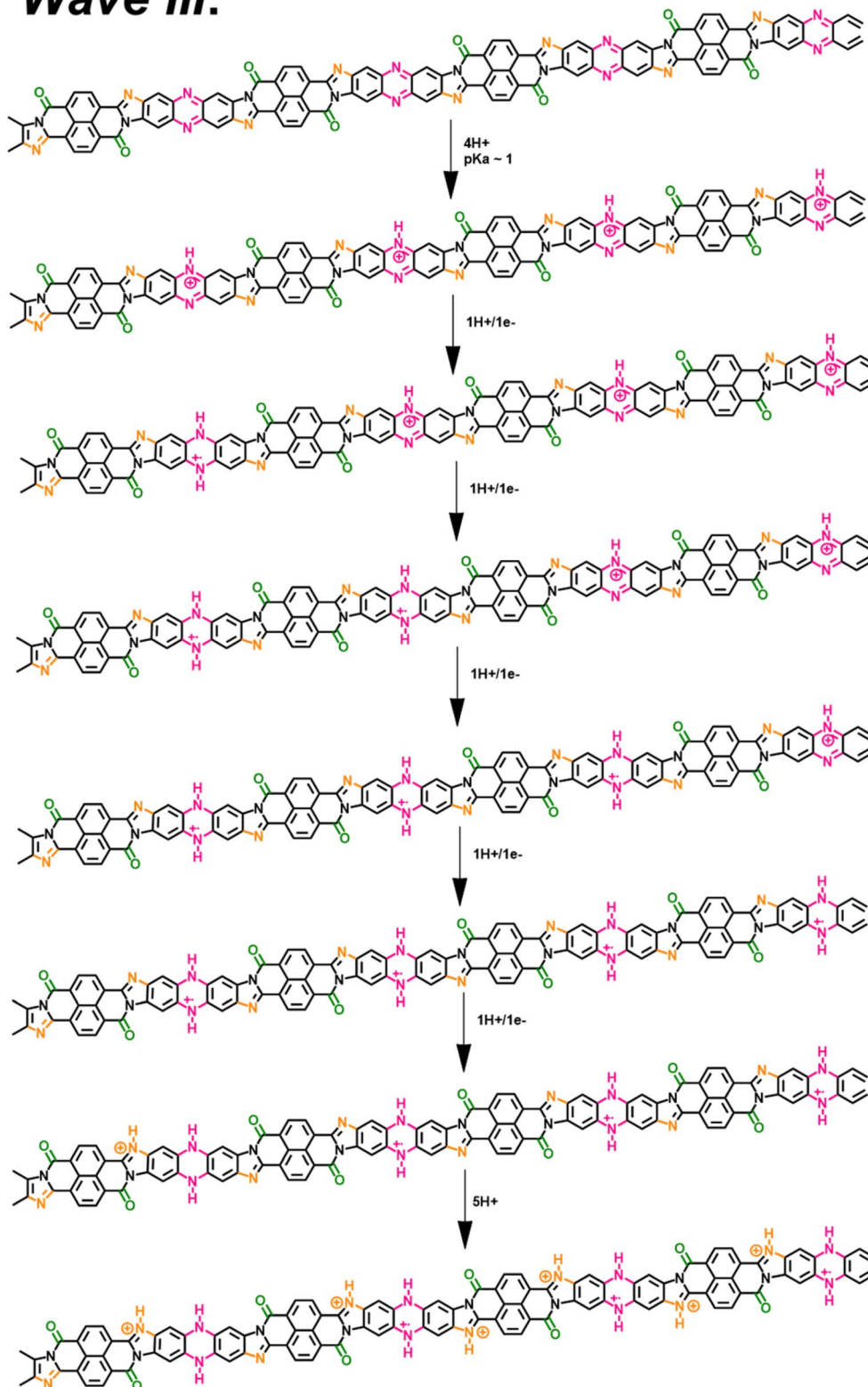
Scheme 4 A two-proton/one-electron electrochemical doping reaction (wave III) of BBL-P consisting of a 1H + /1e - transferred at each phenazine imine sites accompanied by 1H + at the naphthalene imine sites.
