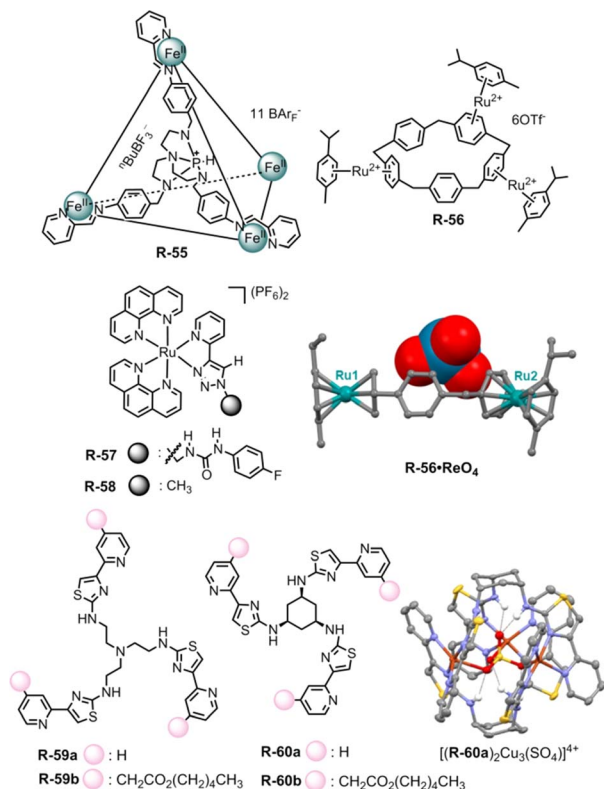
Fig. 19 Chemical structure of the receptors R-55 to R-60 , crystal structure of the R-56 ·ReO 4 complex (data from the Cambridge Crystallographic Data Centre [CCDC # 1951588] 91 ) and self-assembled structure of [( R-60a ) 2 Cu 3 (SO 4 )] 4+ . (Reproduced from ref. 93. Copyright 2020, Wiley-VCH GmbH.)
