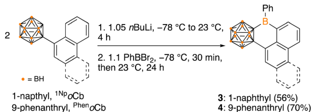
Scheme 1 Synthesis of six-membered boracycles 3 and 4 by dehydrobromination.
