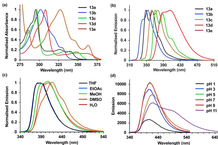
Fig. 3 (a) Absorption spectra of amino acids 13a–13e (5 \mu\text{M} ) in methanol. (b) Normalised emission spectra of amino acids 13a–13e (5 \mu\text{M} ) in methanol. (c) Normalised emission spectra of 13d (5 \mu\text{M} ) in various solvents. (d) Emission spectra of 13d (5 \mu\text{M} ) at various pH.
