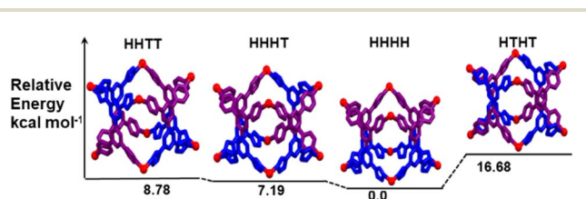
Fig. 3 Energy level diagram with the DFT [B3LYP/LanL2DZ, 6-31G] geometry optimized structures in the gas phase for the four possible linkage isomers of the [\text{Pd}_8(\text{L}^{\text{un}})_4]^{16+} complex.
