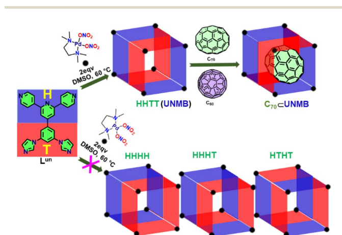
Scheme 1 Schematic presentation of the synthesis of unsymmetrical molecular barrel UNMB, and its selective encapsulation of C 70 .
