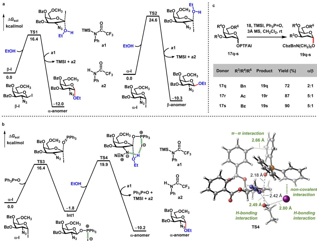
Scheme 6 (a) Energy profiles for the \text{S}_{\text{N}}2 reaction of the alcoholic acceptor with \alpha -iodide and \beta -iodide; (b) energy profile for the \text{Ph}_3\text{P}=\text{O} promoted \text{S}_{\text{N}}2 nucleophilic reaction of \alpha -iodide with alcoholic acceptors; (c) glycosylation between 2-deoxy glycosyl PTFAI donors 17q-s and 18 with TMSI and \text{Ph}_3\text{P}=\text{O} .
