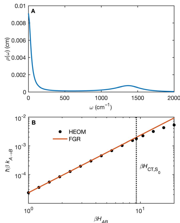
Fig. 6 (A) The coarse-grained model spectral distribution for the ^5\text{CT} \rightarrow \text{S}_0 transition, consisting of a low frequency Debye contribution \rho_{\text{D}}(\omega) = (1/2\pi)/(1 + (\omega/\omega_{\text{D}})^2) , with \beta\omega_{\text{D}} = 0.1831 , and an under-damped Brownian oscillator contribution \rho_{\text{BO}}(\omega) = (1/2\pi)\gamma\Omega^2/((\omega^2 - \Omega^2)^2 + \gamma^2\omega^2) with \beta\gamma = 4 and \beta\Omega = 6.76 . The reorganization energy for the Brownian oscillator portion is \beta\lambda = 8.6780 and for the Debye portion is \beta\lambda = 10.1459 . (B) The rate constant from HEOM calculations for the coarse-grained spectral density as a function of H_{\text{AB}} together with the FGR predictions. The value of H_{\text{AB}} for the ^5\text{CT} \rightarrow \text{S}_0 transition is also indicated. Calculations were performed using the heom-lab code 58 using the HEOM truncation scheme from ref. 59.
