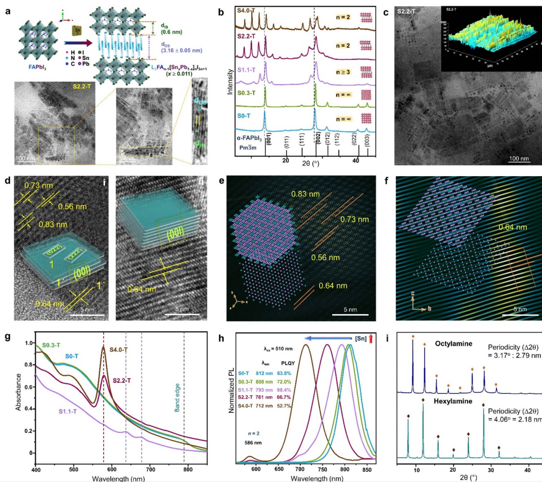
Fig. 6 (a) Schematic showing the transformation of 3D FAPbI 3 NCs to 2D RP superlattice of L 2 FA n-1 [Sn x Pb 1-x ] n I 3n+1 ( x \geq 0.011 ), and the TEM analysis of S2.2-T NPL superlattice. Sequentially magnified TEM images show the superlattice structure, and its correlation with d = d_{\text{IB}} + d_{\text{OS}} = 4.35 \pm 0.06 nm. IB and OS represent the inorganic block with n = 2 , and the organic spacer, respectively. (b) PXRD patterns with increasing Sn/Pb ratio, illustrating the gradual phase change from cubic NCs to 2D RP NPLs. (c) TEM image, and AFM image (inset) for the S2.2-T superlattice. (d) TEM images and schematics showing the NPL stacking with (i), and without (ii) edge offset. FFT mask filter analysis of the NPLs with (e) edge offset stacking, and (f) perfect stacking. The lower left insets show the model crystal lattice of a single NPL, and upper left insets demonstrate the stacking of four lattice planes. (g) Optical absorbance spectra, and (h) PL spectra ( \lambda_{\text{ex}} = 510 nm) of S0-T, S0.3-T, S1.1-T, S2.2-T and S4.0-T. (i) XRD patterns of the RP NPLs ( x = 0.022 , n = 2 ) with hexylamine and octylamine as the spacer. Reproduced with permission from ref. 89, copyright (2023) WILEY-VCH Verlag GmbH & Co. KGaA, Weinheim.
