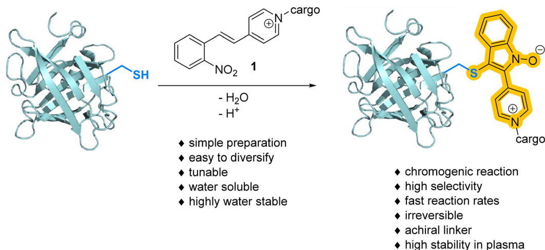
Scheme 1 The reaction of a cysteine sulphydryl group with a nitro-styryl electrophile results in an irreversible bioconjugation that is accompanied by a large bathochromic shift.
