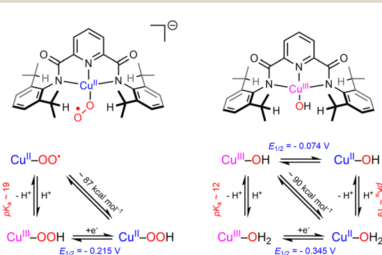
Scheme 6 Comparison of the thermodynamic properties of [(L)Cu^{II}(\eta^1-O_2)]^- and [(L)Cu^{III}(OH)] using the same bis(arylcarboxamido)-pyridine ligand. Adapted from ref. 103.
