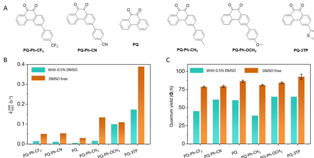
Fig. 2 Overview of the first order reaction rate ( k_{\text{obs}} ) and photoreaction quantum yield ( \Phi_p ) of the PQ-ERA photoclick reaction system. (A) Structures of the investigated PQs; (B) The k_{\text{obs}}(390) and (C) \Phi_p of PQ-ERA photoclick reaction. Cyan: with DMSO, orange: DMSO-free, respectively. NB: k_{\text{obs}} and \Phi_p are measured under different conditions (for more detailed information see ESI,† Section 2.1 and 2.2).
