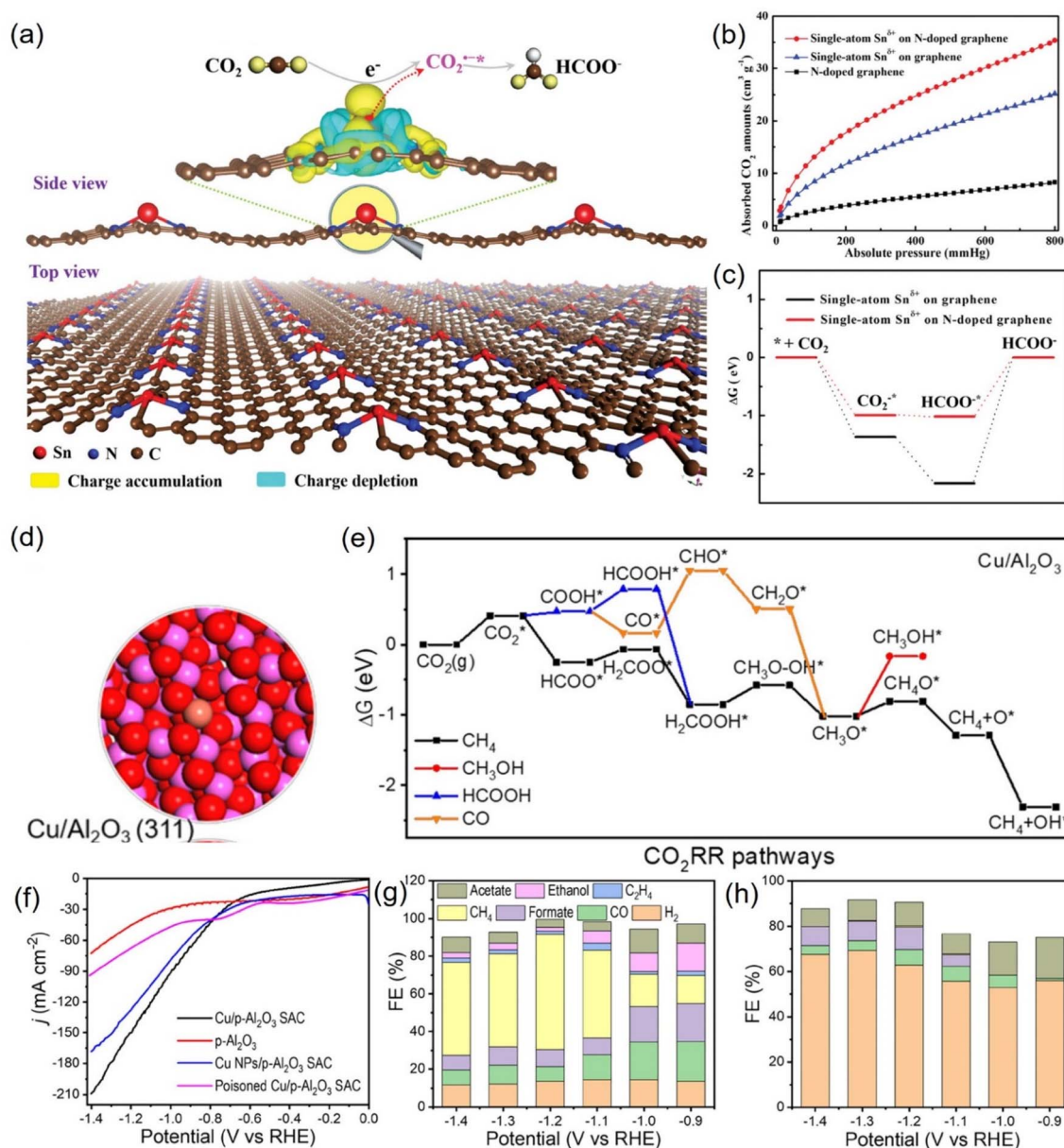
Fig. 20 (a) 3D differential charge densities of single-atom \text{Sn}^{\delta+} on N-doped graphene for \text{CO}_2 reduction to formate. (b) \text{CO}_2 adsorption isotherms and (c) calculated free energy diagrams. (d) Electronic structure of \text{Cu}/\text{Al}_2\text{O}_3 SAC. (e) Calculated free-energy diagrams for the \text{CO}_2\text{RR} over \text{Cu}/\text{Al}_2\text{O}_3 SAC. (f) LSV curves and FEs of various products for (g) \text{Cu}/\text{p-Al}_2\text{O}_3 SAC and (h) \text{p-Al}_2\text{O}_3 . (a-c) Reproduced with permission. 227 Copyright 2019, Wiley-Blackwell. (d-h) Reproduced with permission. 229 Copyright 2021, American Chemical Society.
