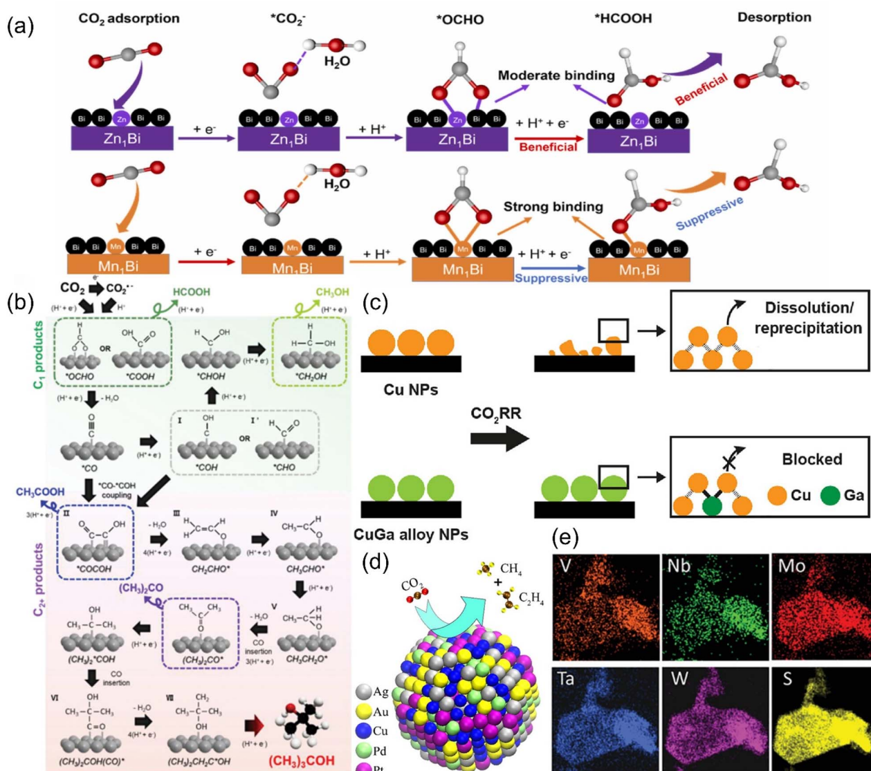
Fig. 21 (a) A proposed reaction mechanism for \text{CO}_2\text{R} to formate on SAA-Zn 1 Bi and SAA-Mn 1 Bi. (b) A probable mechanism for \text{CO}_2\text{R} to (\text{CH}_3)_3\text{COH} . (c) Illustration of the \text{CO}_2\text{RR} stabilization mechanism on CuGa alloy NPs. (d) Schematic of the catalysis reaction on AuAgPtPdCu. (e) EDS maps of (\text{MoWVNbTa})\text{S}_2 . (a) Reproduced with permission. 233 Copyright 2023, Elsevier Ltd. (b) Reproduced with permission. 236 Copyright 2023, Wiley-VCH GmbH. (c) Reproduced with permission. 237 Copyright 2023, American Chemical Society. (d) Reproduced with permission. 240 Copyright 2020, American Chemical Society. (e) Reproduced with permission. 241 Copyright 2021, Wiley-VCH GmbH.
