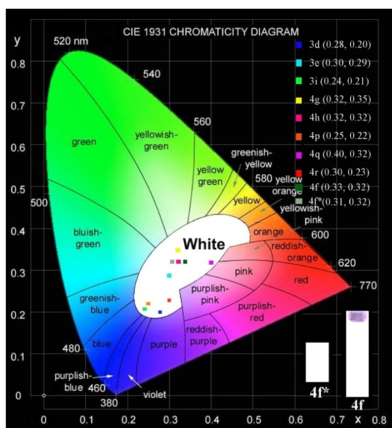
Fig. 4 Chromatic coordinates. Commission Internationale de l'Éclairage (CIE) coordinates of 3d (0.28, 0.20), 3e (0.30, 0.29), 3i (0.24, 0.21), 4g (0.32, 0.35), 4h (0.32, 0.32), 4p (0.25, 0.22), 4q (0.40, 0.32), and 4r (0.30, 0.23) in \text{CH}_2\text{Cl}_2 , respectively.
