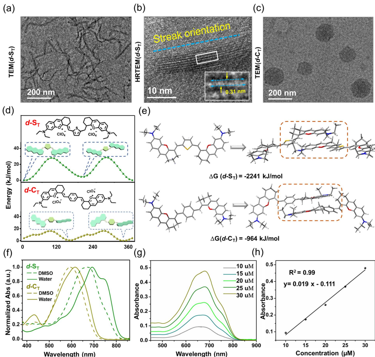
Fig. 1 (a and c) TEM images of the self-assembled structures of d-S_T and d-C_T in H_2O (10 \mu M ) after 30 min. (b) The streak orientation and lattice distance of d-S_T (10 \mu M ) by high-resolution TEM. (d) Molecular energy and corresponding geometries in different conformational states of d-S_T and d-C_T . (e) Proposed packing models of d-S_T (10 \mu M ) and d-C_T (10 \mu M ) with the corresponding binding energy ( \Delta G ). (f) Absorption spectra of d-S_T and d-C_T in DMSO and water. (g) Absorption spectra of d-S_T with different concentrations (10–30 \mu M ). (h) Molar absorption coefficient ( \epsilon ) of d-S_T .
