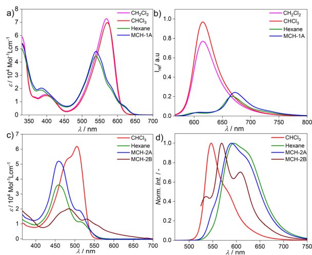
Fig. 1 Solvent-dependent absorption studies of: (a) compound 1 , (c) compound 2 and solvent-dependent fluorescence studies of: (b) compound 1 , \lambda_{exc} = 510 nm and (d) compound 2 , \lambda_{exc} = 470 nm at 298 K, c = 2 \times 10^{-5} M.
