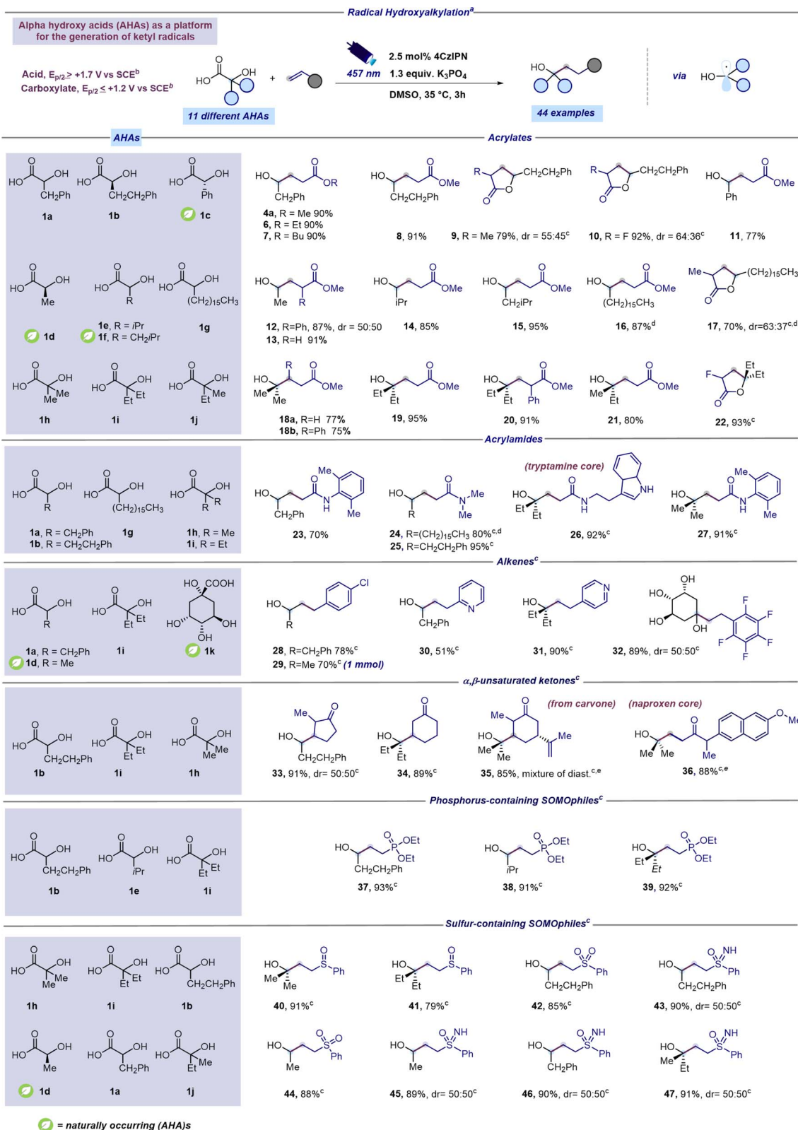
Scheme 1 Scope for radical hydroxyalkylation with AHAs. a Reaction performed under optimized reaction conditions: unsaturated acceptor (0.23 mmol, 1 equiv.), \alpha -hydroxy acid (1.3 equiv.), K 3 PO 4 (1.3 equiv.), and 4CzIPN (2.5 mol%) in DMSO (0.46 M) as the solvent. The mixture was irradiated with 457 nm light (40 W) for 3 h unless otherwise specified. Isolated yields are reported. b Oxidation potentials measured by cyclic voltammetry. Refer to the ESI† for further details. c A reaction time of 16 hours was used instead of 3 hours. d Reaction performed using a concentration of 0.15 M instead of 0.46 M. e Reaction performed using 128 W instead of 40 W. Abbreviations: Ph, phenyl; Me, methyl; i Pr, isopropyl; Et, ethyl.
