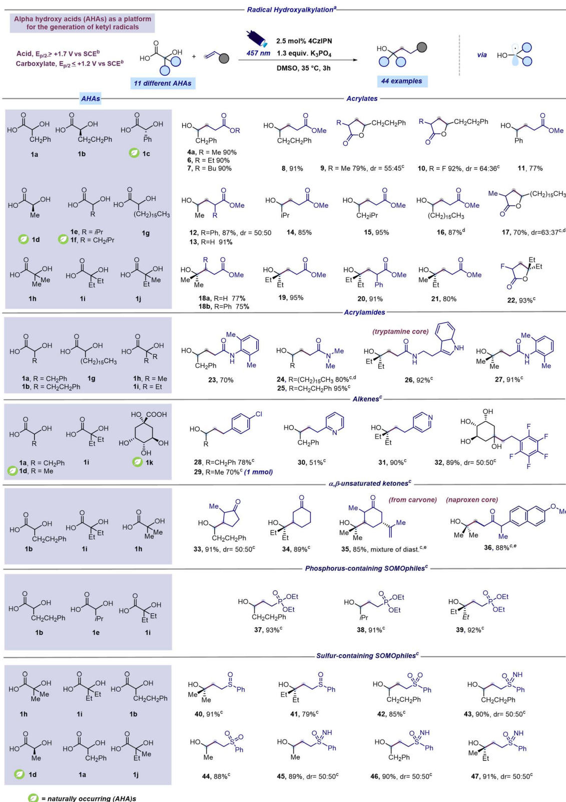
Scheme 1 Scope for radical hydroxyalkylation from AHAs. a Reaction performed under optimized reaction conditions: unsaturated acceptor (0.23 mmol, 1 equiv.), \alpha -hydroxy acid (1.3 equiv.), \text{K}_3\text{PO}_4 (1.3 equiv.), and 4CzIPN (2.5 mol%) in DMSO (0.46 M) as the solvent. The mixture was irradiated with 457 nm light (40 W) for 3 h unless otherwise specified. Isolated yields are reported. b Oxidation potentials measured by cyclic voltammetry. Refer to the ESI† for further details. c A reaction time of 16 hours was used instead of 3 hours. d Reaction performed using a concentration of 0.15 M instead of 0.46 M. e Reaction performed using 128 W instead of 40 W. Abbreviations: Ph, phenyl; Me, methyl; i\text{Pr} , isopropyl; Et, ethyl.
