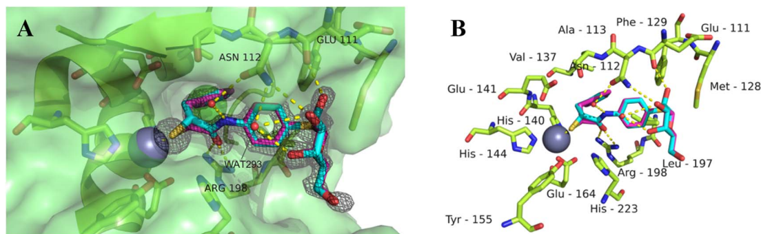
Fig. 6 Crystal structure of 11 in complex with LasB (PDB: 7Z68). (A) Cartoon representation of LasB with a transparent surface (green) and ligated 11 (cyan (R), pink (S)). The amino acids of LasB forming the binding site are represented as sticks. The gray isomesh represents the polder map of 11 contoured at 3\sigma . (B) Stick representation of the LasB binding site with bound 11 . Polar interactions between LasB and 11 are highlighted by dashed lines (color code: oxygen = red, nitrogen = blue, sulfur = yellow, and red spheres = water).
