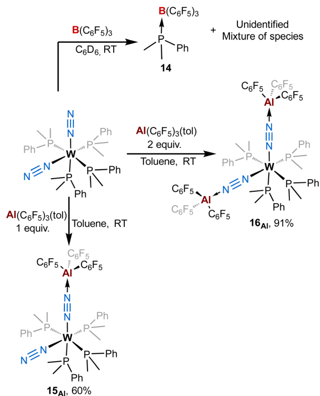
Scheme 4 Reactivity of [\text{M}(\text{PMe}_2\text{Ph})_4(\text{N}_2)_2] ( \text{M} = \text{W} or \text{Mo} ) complexes with (top) \text{B}(\text{C}_6\text{F}_5)_3 and (bottom) \text{Al}(\text{C}_6\text{F}_5)_3(\text{tol}) .
