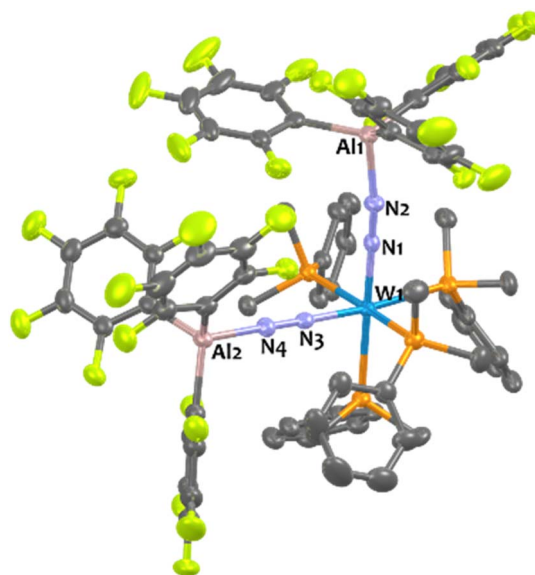
Fig. 8 Solid-state structure of 16 Al . Ellipsoids are represented with 30% probability. Hydrogen atoms have been omitted for clarity. Selected bond distances (Å) and angles (°): \text{Al}_1\text{-N}_2 1.915(3), \text{Al}_2\text{-N}_4 1.891(3), \text{W}_1\text{-N}_1 1.917(3), \text{W}_1\text{-N}_3 1.906(3), \text{N}_1\text{-N}_2 1.149(4), \text{N}_3\text{-N}_4 1.150(4), \text{W}_1\text{-N}_1\text{-N}_2 179.2(3), \text{W}_1\text{-N}_3\text{-N}_4 177.5(3), \text{N}_1\text{-W}_1\text{-N}_3 91.34(1), \text{Al}_1\text{-N}_2\text{-N}_1 168.5(3), \text{Al}_2\text{-N}_4\text{-N}_3 179.1(3).
