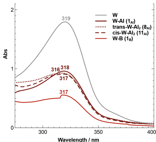
Fig. 9 Absorption spectra of \text{trans-}[\text{W}(\text{depe})_2(\text{N}_2)_2] (W, grey line), \text{trans-}[\text{W}(\text{depe})_2(\text{N}_2)(\mu\text{-N}_2\text{-Al}(\text{C}_6\text{F}_5)_3)] ( \text{W-Al} , crimson line), \text{trans-}[\text{W}(\text{depe})_2\{\mu\text{-N}_2\text{-Al}(\text{C}_6\text{F}_5)_3\}_2] ( \text{trans-W-Al}_2 , dotted crimson line), \text{cis-}[\text{W}(\text{depe})_2\{\mu\text{-N}_2\text{-Al}(\text{C}_6\text{F}_5)_3\}_2] ( \text{cis-W-Al}_2 , dashed crimson line), and \text{trans-}[\text{W}(\text{depe})_2(\text{N}_2)(\mu\text{-N}_2\text{-B}(\text{C}_6\text{F}_5)_3)] ( \text{W-B} , red line). The concentration of each sample is about 30 \mu\text{M} .
