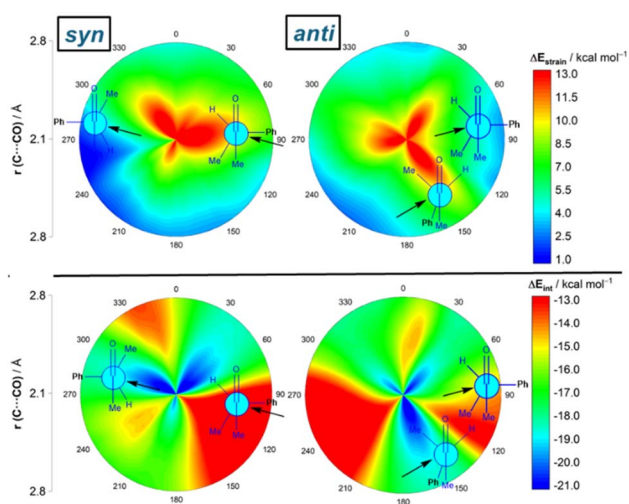
Fig. 7 2D-activation strain diagrams of the possible cyanide additions to ( S )-3-phenylbutan-2-one leading to the corresponding syn (left) and anti (right) reaction products. Strain energy (top) and interaction energy (bottom). All data were computed at the ZORA-M06-2X/TZ2P//M06-2X-6-311+G(d) level.
