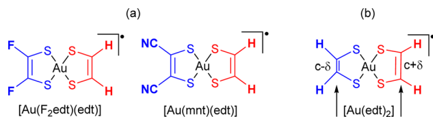
Scheme 4 Model complexes theoretically investigated with (a) [\text{Au}(\text{R,Redt})(\text{edt})]^+ ( \text{R}=\text{F}, \text{CN} ) complexes, (b) [\text{Au}(\text{edt})_2]^+ complexes with constrained C=C bonds.
