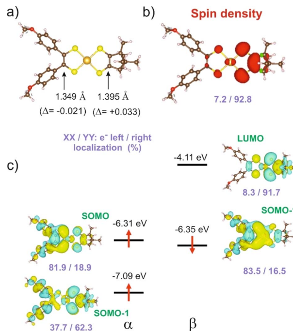
Fig. 5 [\text{Au}(\text{OC}_4)(D\text{-bordt})]^+ complex: (a) C=C optimized bond lengths, (b) spin density, and (c) spin-orbitals around the SOMO. The pairs of violet numbers indicate the left/right distribution (%) of the spin density in (b) or the electron distribution in a given spin-orbital in (c). In (a) the values in parenthesis are the bond length changes with respect to the corresponding symmetric complexes.
