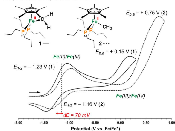
Fig. 2 (A) Synthesis of [\mathbf{1}]^+ and \text{C}(\text{sp}^3)\text{-C}(\text{sp}^3) coupled products. (B) Cyclic voltammograms for 1 and 2 .
