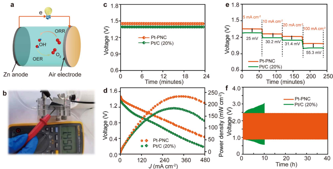
Fig. 6 ZAB application of Pt-PNC. (a) Schematic illustration of ZAB. (b) OCP photograph of Pt-PNC-based ZAB. (c) Open circuit voltage curves. (d) Discharge curves and corresponding peak power density plots. (e and f) Galvanostatic discharge curves at varying current densities (5, 10, 20, and 100 mA cm -2 ) and cycling stability test at 10 mA cm -2 for the ZABs with different catalysts.
