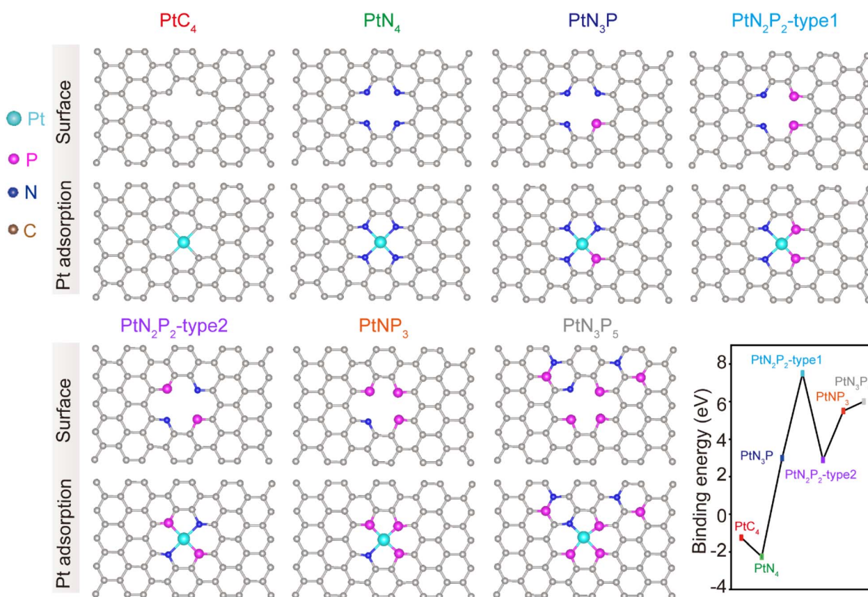
Fig. 1 Prediction of the structural stability of Pt single atoms with different first coordination environment and calculated binding energy of Pt atom anchored on the doped-graphene ( PtC_4 , PtN_4 , PtN_3P , PtN_2P_2 -type 1, PtN_2P_2 -type 2, PtNP_3 , PtN_3P_5 ) monolayer. All energies are given in eV.
