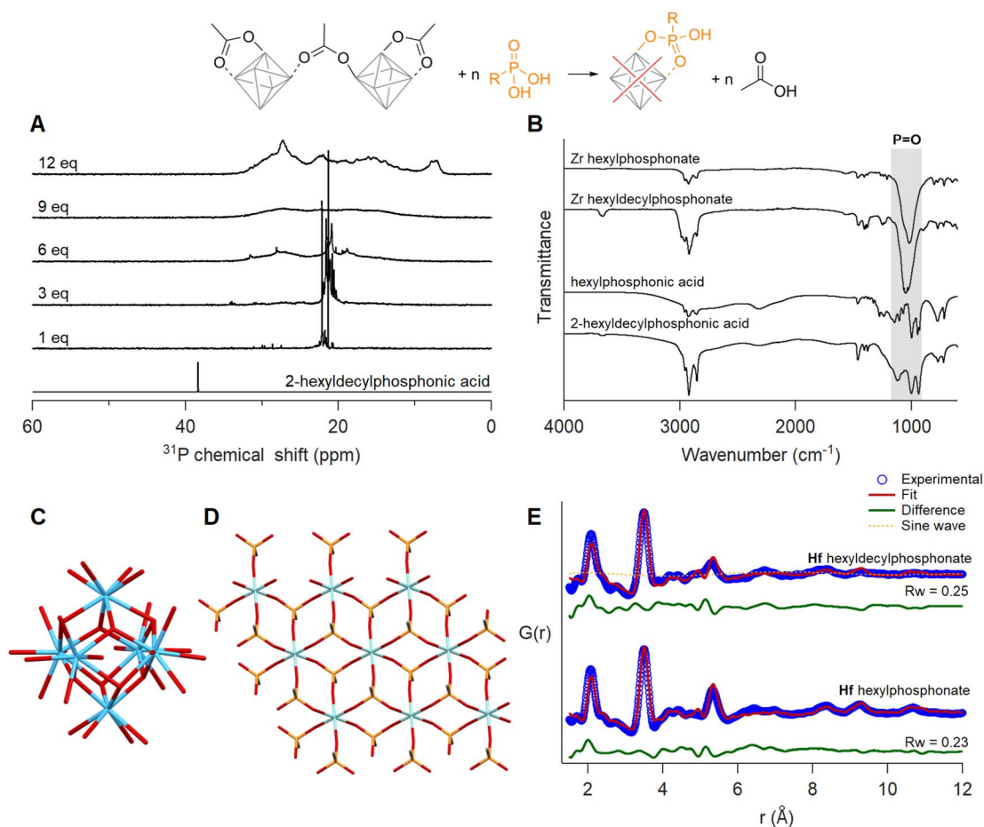
Fig. 7 Ligand exchange of Zr12 -acetate with 2-hexyldecylphosphonic acid. (A) 31 P spectra of the titration, with the reference spectrum of 2-hexyldecylphosphonic acid with one equivalent of acetic acid added. The concentration of the cluster was 20 \text{mg mL}^{-1} in \text{CDCl}_3 . (B) IR spectra of phosphonate exchanged zirconium clusters after isolation and purification. IR spectra of free acids are provided as a reference. (C) Structure model of Hf6 cut from the crystal structure of Hf12 -acetate. (D) Structure of a 3 \times 3 layer zirconium phenylphosphonate (JPCDS: 44-2000). Cyan and blue atoms represent zirconium and hafnium, respectively; all other atoms follow conventional CPK coloring. Only the carbon bonded to phosphonate is shown, and the rest of the phenyl ring is omitted for clarity. (E) Dual-phase PDF fit for phosphonate exchanged Hf clusters with a 3 \times 3 layer of Hf phenylphosphonate (contains 9 hafnium atoms in total) and Hf6 chelating bridging acetate.
