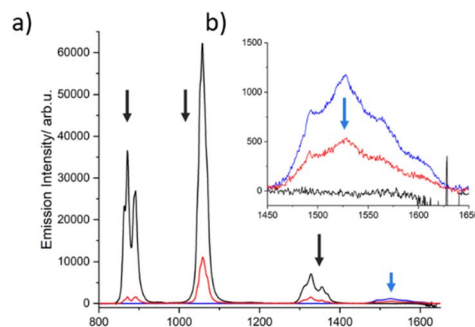
Fig. 6 Emission spectra ( \lambda_{exc} = 400 nm) of iso-absorbant solutions of complexes (1) (black trace), (2) (blue trace), and (3) (red trace) in MeOD- d_4 : DMSO- d_6 (1 : 1) solution at room temperature (a) with the corresponding Er^{3+} emission zoom (b).
