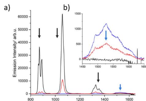
Fig. 6 Emission spectra ( \lambda_{exc} = 400 nm) of iso-absorbant solutions of complexes ( 1 ) (black trace), ( 2 ) (blue trace), and ( 3 ) (red trace) in MeOH- d_4 : DMSO- d_6 (1 : 1) solution at room temperature (a) with the corresponding Er^{3+} emission zoom (b).
