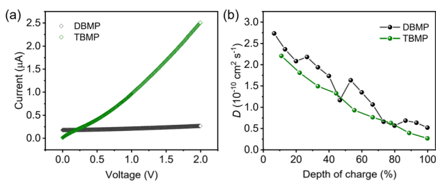
Fig. 4 Ionic and electronic conductivities of DBMP and TBMP. (a) I - V plot of DBMP and TBMP pellets for measuring the electrical conductivity. (b) The ion diffusion coefficient calculated from the GITT profiles of DBMP and TBMP based electrodes.
