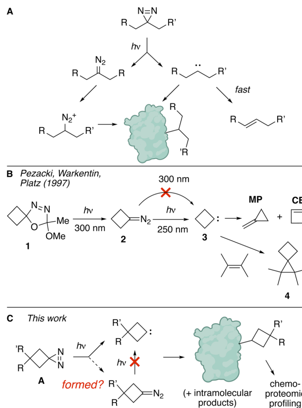
Fig. 1 (A) 'Linear' diazirines produce both carbene and diazo compounds upon photolysis. The carbene products are susceptible to intramolecular 1,2 H-shift. A primary labeling pathway involves protonation of the diazo compound and subsequent alkylation. (B) Prior studies showed spirocyclic oxadiazoline ketal 1 to be a precursor to diazocyclobutane 2 , which can be used to produce cyclobutylidene 3 at 250 nm irradiation, but not at wavelengths longer than 300 nm with standard light sources. (C) We demonstrate that cyclobutanediazirines A produce carbene products upon photolysis. The diazocyclobutane is not observed, and does not serve as a photochemical precursor to the carbene.
