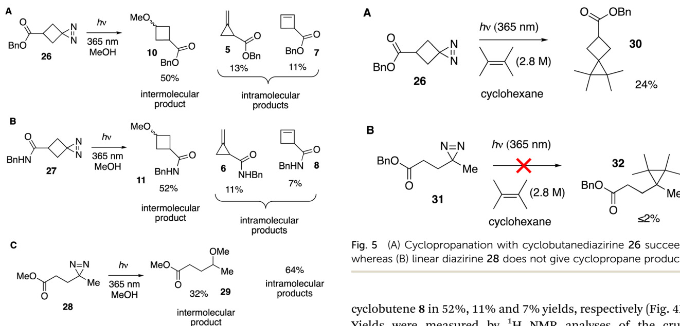
Fig. 4 (A and B) Photolysis of spirocyclic diazirines in \text{MeOH} produces intermolecular products 10 and 11 in >50% yield, along with methylenecyclopropane and cyclobutene products of unimolecular rearrangement. (C) Photolysis of linear diazirine 28 produces intermolecular product 29 in 32% yield, along with 64% yield of alkene products of unimolecular rearrangement.
