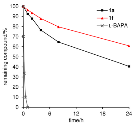
Fig. 7 Proteolytic stability of 1a and 1f (71 \mu M) against papain (0.81 mM). The amount of remaining compound (%) was analyzed during 24 h incubation. L-BAPA = benzoyl-L-arginine- p -nitroanilide.
