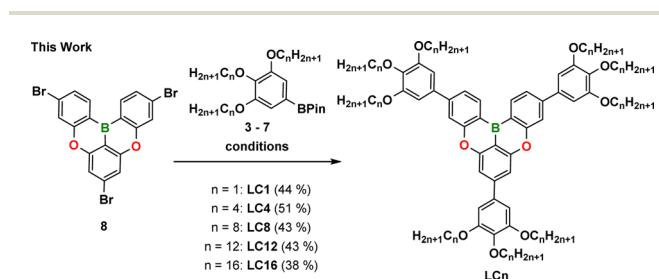
Scheme 1 Synthetic procedure for the preparation of the library of LC n compounds possessing different chain lengths varying from -\text{CH}_3 to \text{C}_{16}\text{H}_{33} . Conditions: \text{Pd}(\text{PPh}_3)_4 (0.15 equiv.), 3–7 (3.5 equiv.), \text{Cs}_2\text{CO}_3 (5 equiv.), toluene: \text{H}_2\text{O} (10 : 1, v : v), 110 °C, 18 h.
