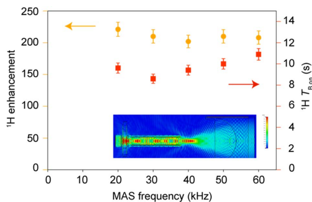
Fig. 6 Enhancement factors and polarization build-up times of 10 mM M-TinyPol(OH) 4 in a bulk solution of d_8 -glycerol/ \text{D}_2\text{O}/\text{H}_2\text{O} 60/30/10 (v/v/v), as a function of MAS frequency. Enhancements values were measured at 18.8 T from proton NMR spectra, in a 0.7 mm zirconia rotor at a sample temperature of 110 \pm 5 K. The inset shows the microwave distribution within the rotor predicted by finite-element simulations.
