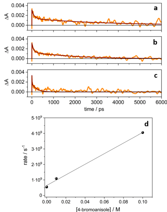
Fig. 4 Normalized temporal evolution of ΔA measured at 1440 nm (orange line) for a degassed solution of 4CzIPN •- (a) and in the presence of 0.01 M (b) and 0.1 M (c) 4-bromoanisole. (d) Rate constant of the ΔA decay at 1440 nm as a function of the concentration of 4-bromoanisole.
