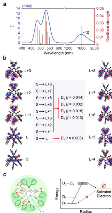
Fig. 6 (a) The calculated absorption spectrum of 4DPAIPN^{\bullet-} , with a different scale use for intensity and absorption profile at long wavelengths. (b) Frontier orbitals involved in the main excitations with D_2 – D_5 being electron transfer from phenyl core to peripheral units. (c) Schematics illustrating the charge carrier character of the D_2 – D_5 states that facilitates electron transfer to solvent and create a barrier for the back electron transfer. The energy levels are represented to highlight the distance of the negative charge (radius r ) from the centre of the molecule in the respective state.
