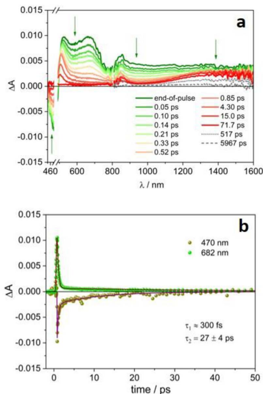
Fig. 3 Transient absorption spectra at different delays of a degassed acetonitrile solution of 4CzIPN •- (a) and the corresponding ΔA temporal evolution at significant wavelengths (b). λ ex = 480 nm, A 480 = 0.28, 0.2 cm optical path, 8 μJ per pulse.
