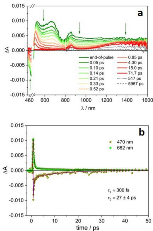
Fig. 3 Transient absorption spectra at different delays of a degassed acetonitrile solution of 4\text{CzIPN}^{\cdot-} (a) and the corresponding \Delta A temporal evolution at significant wavelengths (b). \lambda_{\text{ex}} = 480 \text{ nm} , A_{480} = 0.28 , 0.2 \text{ cm} optical path, 8 \mu\text{J} per pulse.
