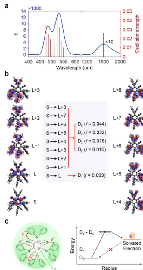
Fig. 6 (a) The calculated absorption spectrum of 4DPAIPN^{\bullet-} , with a different scale for intensity and absorption profile at long wavelengths. (b) Frontier orbitals involved in the main excitations with D_2 – D_5 being electron transfer from phenyl core to peripheral units. (c) Schematics illustrating the charge carrier character of the D_2 – D_5 states that facilitates electron transfer to solvent and create a barrier for the back electron transfer. The energy levels are represented to highlight the distance of the negative charge (radius r ) from the centre of the molecule in the respective state.
