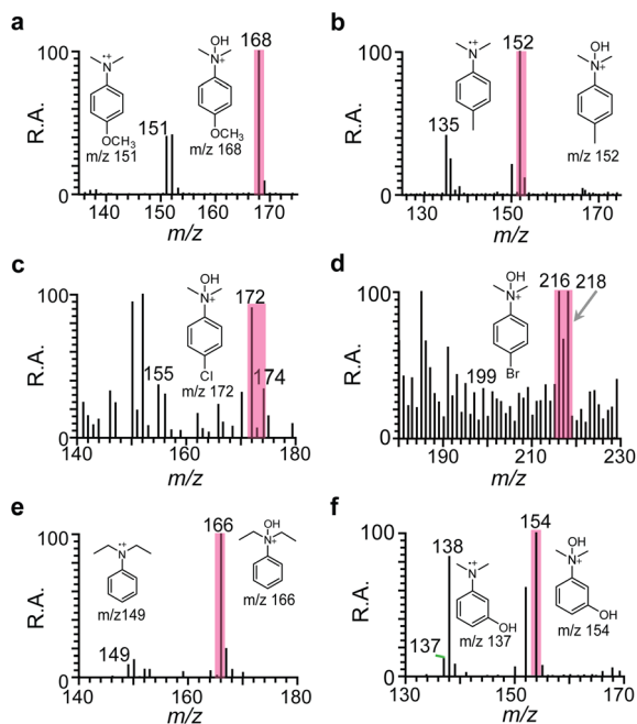
Fig. 3 Reaction scope of the N -hydroxylation reaction of DMA derivatives in water microdroplets. (a) 4-Methoxy- N,N -dimethylaniline. (b) 4-Methyl- N,N -dimethylaniline. (c) 4-Chloro- N,N -dimethylaniline. (d) 4-Bromo- N,N -dimethylaniline. (e) N,N -Diethylaniline. (f) 3-Hydroxy- N,N -dimethylaniline.
