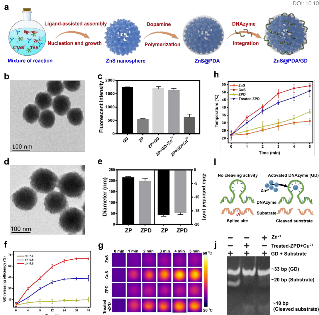
Figure 2. Synthesis and characterization of “copper nanoconsumer” ZPD. (a) Scheme of “copper nanoconsumer” synthesis. (b) TEM image of ZP. (c) Metal ion-mediated adsorption between ZP and GD, probed by fluorescence quenching analysis. (d) TEM image of ZPD. (e) Comparison of diameters and zeta potentials between ZP and ZPD by dynamic light scattering. (f) GD release profile at different pHs. (g) Photothermal imaging under laser irradiation, 808 nm 2 W/cm 2 for 5 min. (h) Photothermal effect analysis by monitoring temperature changing under laser irradiation, 808 nm 2 W/cm 2 for 5 min. (i) Schematic description of DNAzyme-mediated mRNA cleavage. (j) Gel electrophoresis of GD cleaving activity. Each error bar represents the standard deviation of four independent measurements.
