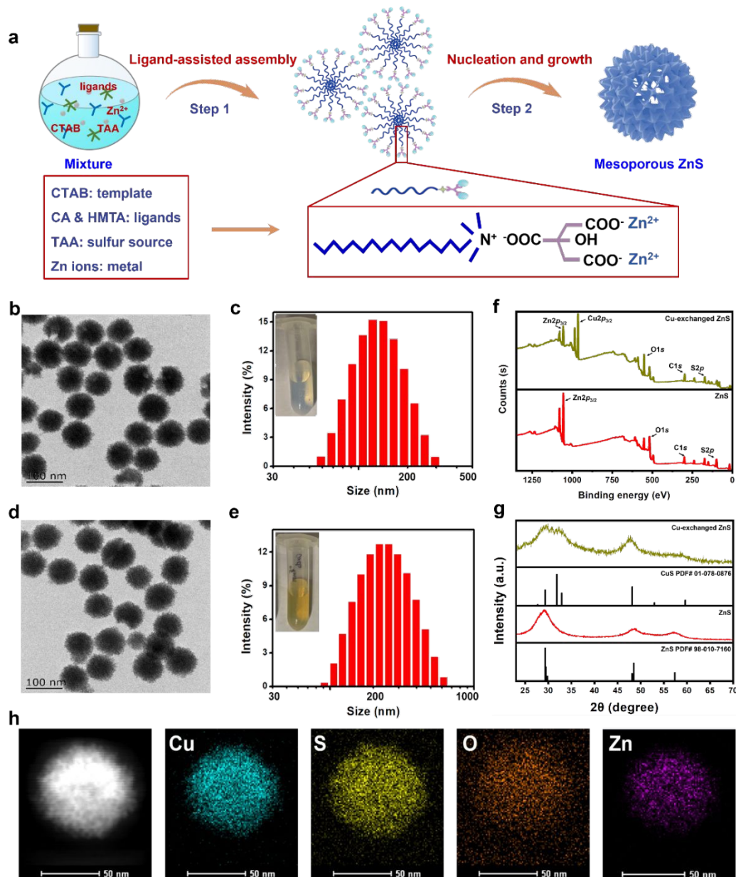
Figure 1. Characterization and copper depleting ability of ZnS. (a) Schematic of mesoporous ZnS nanosphere synthesis. (b) TEM image of ZnS. (c) Size distribution of ZnS. Inset: digital photo of ZnS solution. (d) and (e) TEM image and size distribution of Cu-exchanged ZnS by TEM and DLS. Inset: digital photo of ZnS after Cu depletion. (f) XPS analysis of ZnS and Cu-exchanged ZnS. (g) XRD patterns of ZnS and Cu-exchanged ZnS. (h) Element distribution mapping of ZnS after Cu depletion by HRTEM.
