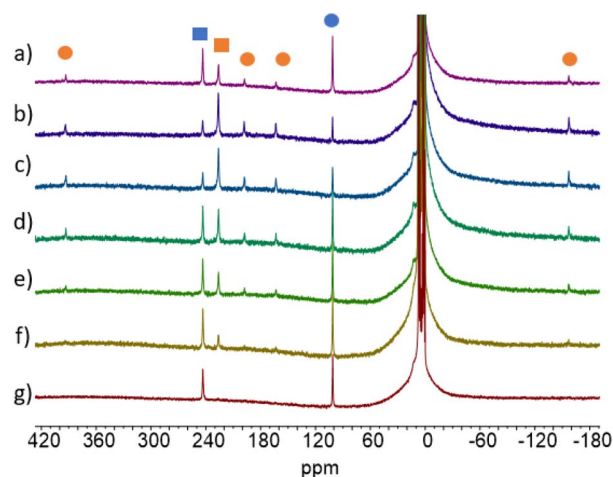
Fig. 6 1 H NMR of 2-Tb at different PPS (after 30 min of irradiation) depending on the wavelength of the irradiation light used (a) t = 0 , (b) \lambda = 370 nm, (c) \lambda = 390 nm, (d) \lambda = 427 nm, (e) \lambda = 467 nm, (f) \lambda = 490 nm, (g) \lambda = 525 nm. Blue is for 2- cis and orange for 2- trans . Squares are for the Cot ligand, and circles are for the Cnt ligand.
