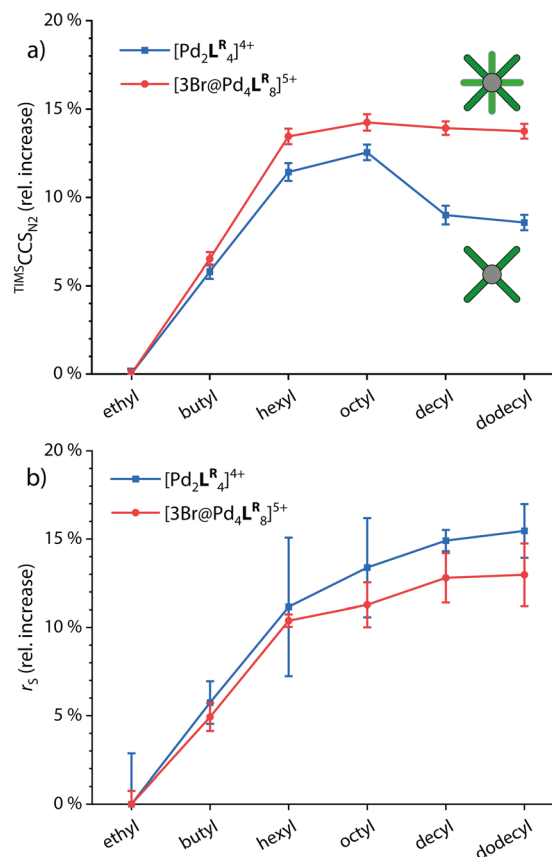
Fig. 3 (a) Relative increase of experimental \text{T}_{\text{IMS}}^{\text{CCS}}\text{N}_2 values and (b) relative increase of solvodynamic radii based on DOSY NMR for the monomeric and double cages (taking the systems with ethyl side chains as a reference).
