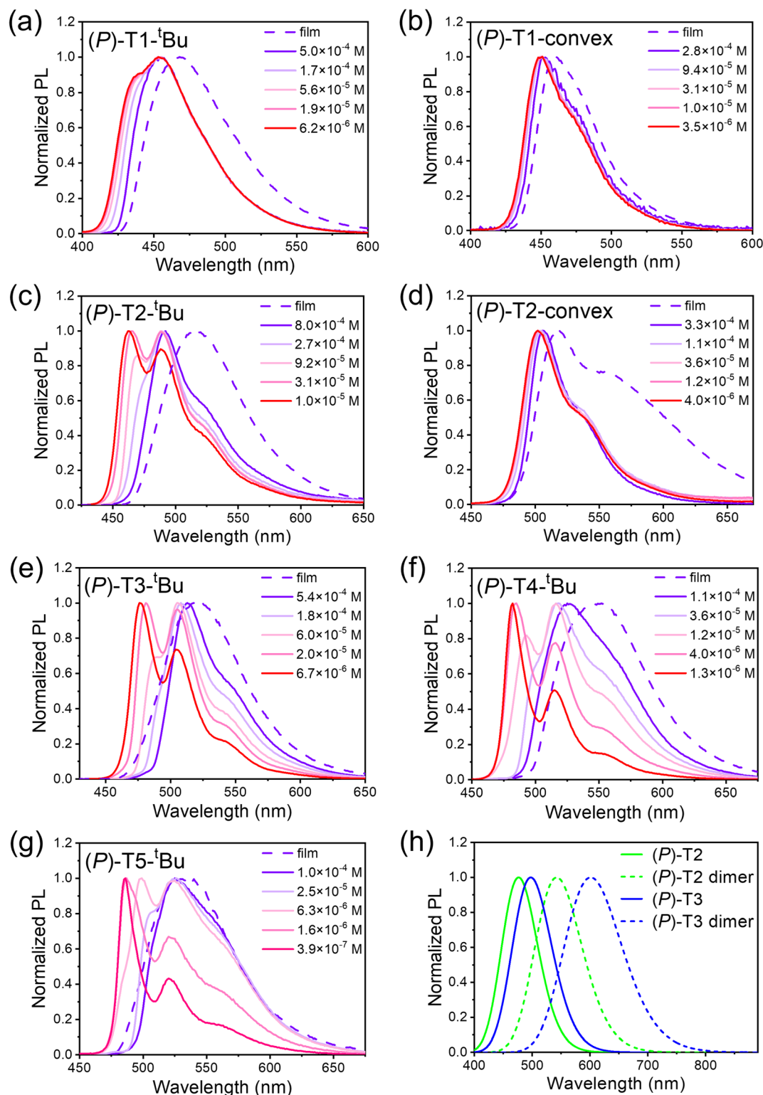
Fig. 6 The photoluminescence spectra for TECHs in solution with different concentration and in film: (a) (P)-T1- t Bu; (b) (P)-T1-convex; (c) (P)-T2- t Bu; (d) (P)-T2-convex; (e) (P)-T3- t Bu; (f) (P)-T4- t Bu; (g) (P)-T5- t Bu. (h) The calculated fluorescence spectra for (P)-T2, (P)-T2 dimer, (P)-T3 and (P)-T3 dimer by TD-DFT theory at the PBE0(D3)/6-31G(d,p) level.
