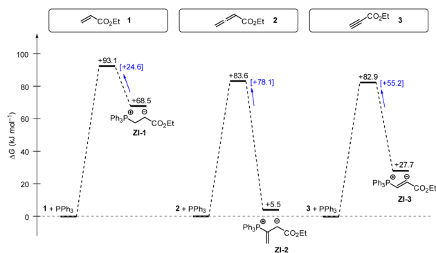
Fig. 16 Gibbs energy profiles for PPh 3 additions to Michael acceptors 1 , 2 and 3 in dichloromethane solution. Experimentally determined Gibbs activation energies \Delta G_{\text{exp}}^\ddagger are combined with quantum-chemically calculated reaction energies \Delta G_{\text{add}} (data from Table 4). Reaction barriers for the retro-additions [ \Delta G_{\text{retro}}^\ddagger ] are given in square brackets.
