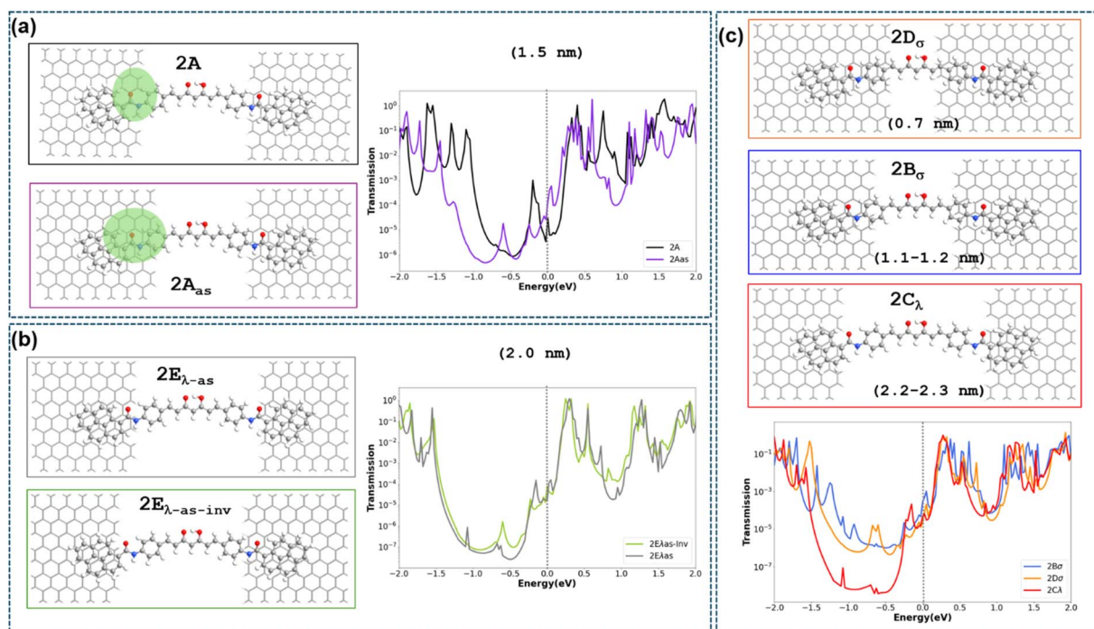
Fig. 3 Seven configuration models: (a) 2A featuring the CCMoid symmetrically coupled to the electrodes with the backbone bridging a nano-gap of 1.5 nm 2A _{as} with an identical gap but asymmetric distribution of the CCMoid (anchoring on one side through the benzene-amide-pyrene moieties) along with the transmission spectrum (in log scale) corresponding to the two configurations; (b) 2E \lambda - _{as} and 2E \lambda - _{as} - _{inv} showing asymmetric coupling of the CCMoid inside the nano-gap of 2 nm and its reverse, respectively accompanied by their transmission spectra. (c) 2B \sigma and 2D \sigma considering symmetric coupling with shorter nano-gaps; 2C \lambda corresponding to symmetric coupling in the largest calculated nano-gap.
