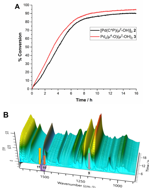
Fig. 6 Model Heck arylation reaction to test Pd 4 cluster 3 against intermediate dinuclear Pd species 2 . (A) Kinetic profiles showing the formation of n -butyl 4-fluorocinnamate 11 (product appearance at 1509 cm -1 ). (B) Temporal IR spectral changes underpinning the kinetic changes shown in A. Formation of 11 at 1509 cm -1 and loss of 1-bromo-4-fluorobenzene 10 at 1484 cm -1 and n -butyl acrylate 9 at 1190 cm -1 (reaction mixture compared with reference standards in NMP solvent).
