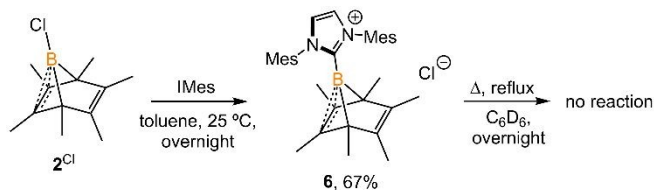
Scheme 3. Synthesis of 6 .
