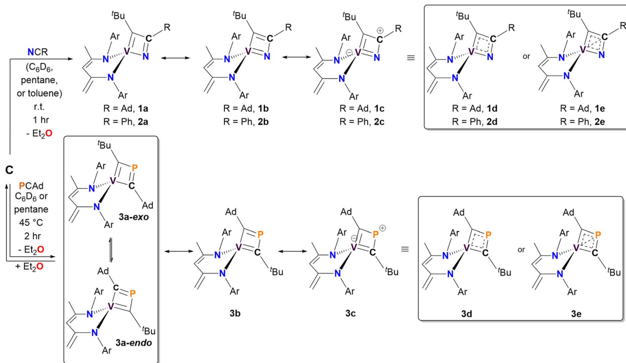
Scheme 1 Synthesis of complexes 1–3 via the [2+2]-cycloaddition of the vanadium alkylidyne C with pnictogen-containing alkynes Pn\equiv CR ( Pn = N, R = Ad \text{ or } Ph ; Pn = P, R = Ad ). Potential resonance structures and charge delocalized structures for each complex are also illustrated.
