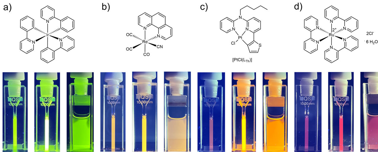
Fig. 4 Structural formulae of fac -tris-(2-phenylpyridine)iridium(III) 49 (a), tricarbonyl(cyano)(1,10-phenanthroline)rhenium(I) 51 , [\text{PtCl}(\text{L-Tr})]^{24} (c) and tris(2,2'-bipyridine)ruthenium(II) dichloride hexahydrate 50 (d). Shown are the corresponding pictures of the cuvettes with each complex (25 \mu\text{M} ) and Asc-Ac (10 mM) in DMF before and after the irradiation in a photoreactor (as observed under UV light, \lambda_{\text{ex}} = 365 \text{ nm} ). Pictures on the right demonstrate the diffusion of fresh oxygen from the headspace after irradiation.
