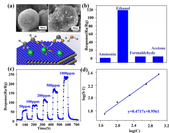
Fig. 9 (a) SEM image of pure \text{MoS}_2 and \text{SnO}_2@\text{MoS}_2 composites as well as the sensing mechanism for the composites, (b) selectivity, (c) dynamic response of the \text{SnO}_2@\text{MoS}_2 sensor as a function of ethanol concentration at 280^\circ\text{C} , and (d) dilogarithm fitting curve of the response–concentration relationship. Reprinted with permission from ref. 76 copyright 2015, The Royal Society of Chemistry.
