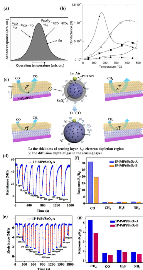
Fig. 18 (a) Temperature-dependent response of MOS sensors toward \text{CO} , (b) temperature-dependent response of the \text{SnO}_2 sensor toward \text{C}_2\text{H}_5\text{OH} (50 ppm), \text{H}_2 (500 ppm), \text{CO} (300 ppm), and \text{CH}_4 (1000 ppm). Reprinted with permission from ref. 151 copyright 2005, Elsevier. (c) Schematic illustration of the \text{CO} -sensing mechanism of \text{PdPt}/\text{SnO}_2 at different working temperatures. The response of the obtained samples toward (d) 50 ppm \text{CO} and (e) 500 ppm \text{CH}_4 at different working temperatures, the response of the \text{PdPt}/\text{SnO}_2 sensors on successive exposure to 1000 ppm \text{CH}_4 and 50 ppm of other hazardous gases in the coal mine at (f) 100 ^{\circ}\text{C} and (g) 320 ^{\circ}\text{C} , respectively. Reprinted with permission from ref. 156 copyright 2019, American Chemical Society.
