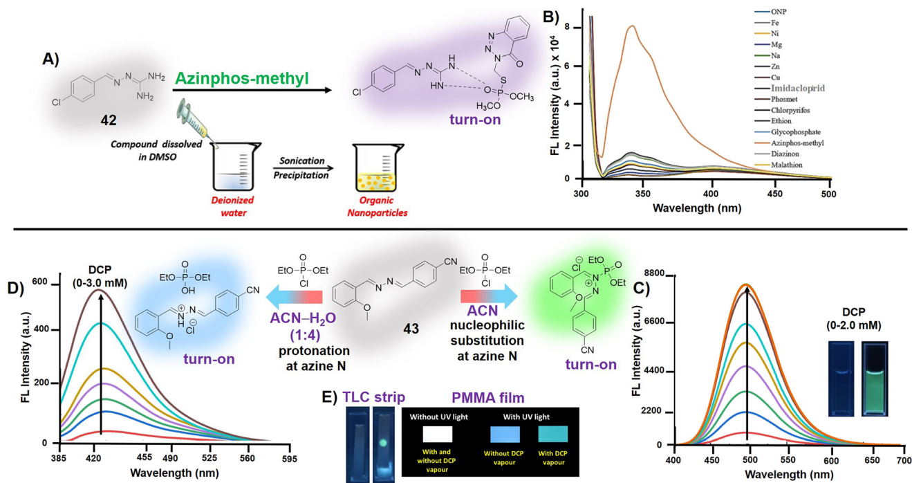
Fig. 7 (A) 1,1-Diaminoazine ( 42 ) as a chemodosensor for organophosphorus pesticide azinphos-methyl; (B) selectivity study of 42 against various OPPs and metal ions (images A and B are adapted with permission from ref. 92. Copyright 2023, Elsevier); salicylaldehyde-based azine ( 43 ) as a dual-mode chemodosimeter for the detection of nerve agent mimic diethylchlorophosphate (DCP) by (C) turn-on emission at 495 nm in ACN due to nucleophilic substitution of the DCP at the azine nitrogen close to the -OMe group giving rise to a new ICT state and (D) turn-on emission at 422 nm due to protonation at the azine nitrogen in an ACN:H 2 O mixture; (E) DCP sensing demonstrated on TLC strips and PMMA polymer film showing green fluorescence emission in the presence of DCP vapors under 365 nm light (images C–E are adapted with permission from ref. 93. Copyright 2021, Elsevier).
