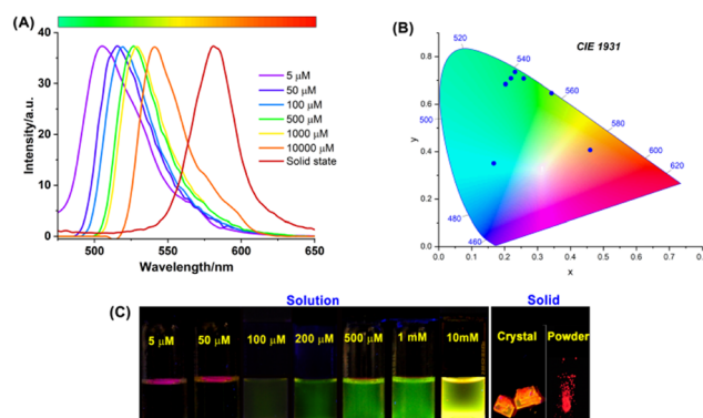
Fig. 3 (A) Normalized fluorescence spectra of 2 at different concentration (5.0 \mu\text{M} to 10 mM) in \text{CH}_3\text{CN} and in the solid state ( \lambda_{\text{ex}} = 485 nm). (B) CIE plot (C) digital photographs of \text{CH}_3\text{CN} solution of probe 2 at different concentrations (5.0 \mu\text{M} to 10 mM) in \text{CH}_3\text{CN} and solid powder, and crystal, showing multicolor fluorescence under UV light illumination (365 nm).
