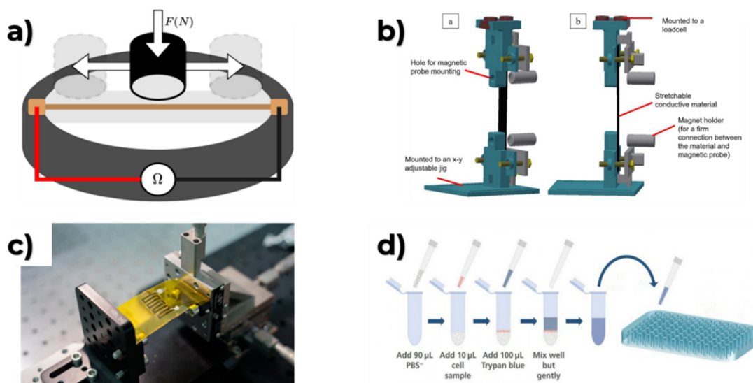
Fig. 7 Equipment for evaluating strain sensor performance. (a) Abrasion tester, 82 (b) tensile machine, 83 (c) electro-mechanical tester for bending test, 84 (d) trypan blue assay. 85
