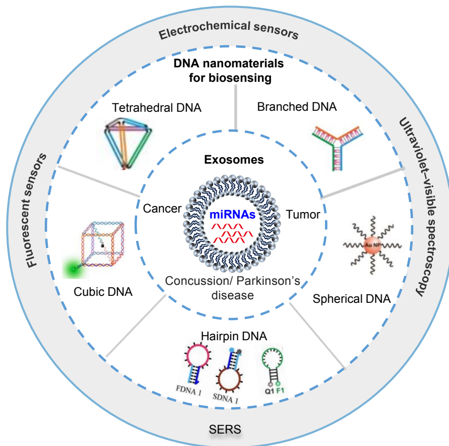
Figure 1. Various DNA nanomaterials for detecting exo-miRs associated with diseases by fluorescent, electrochemical, SERS, and Uv-vis sensing platforms.
