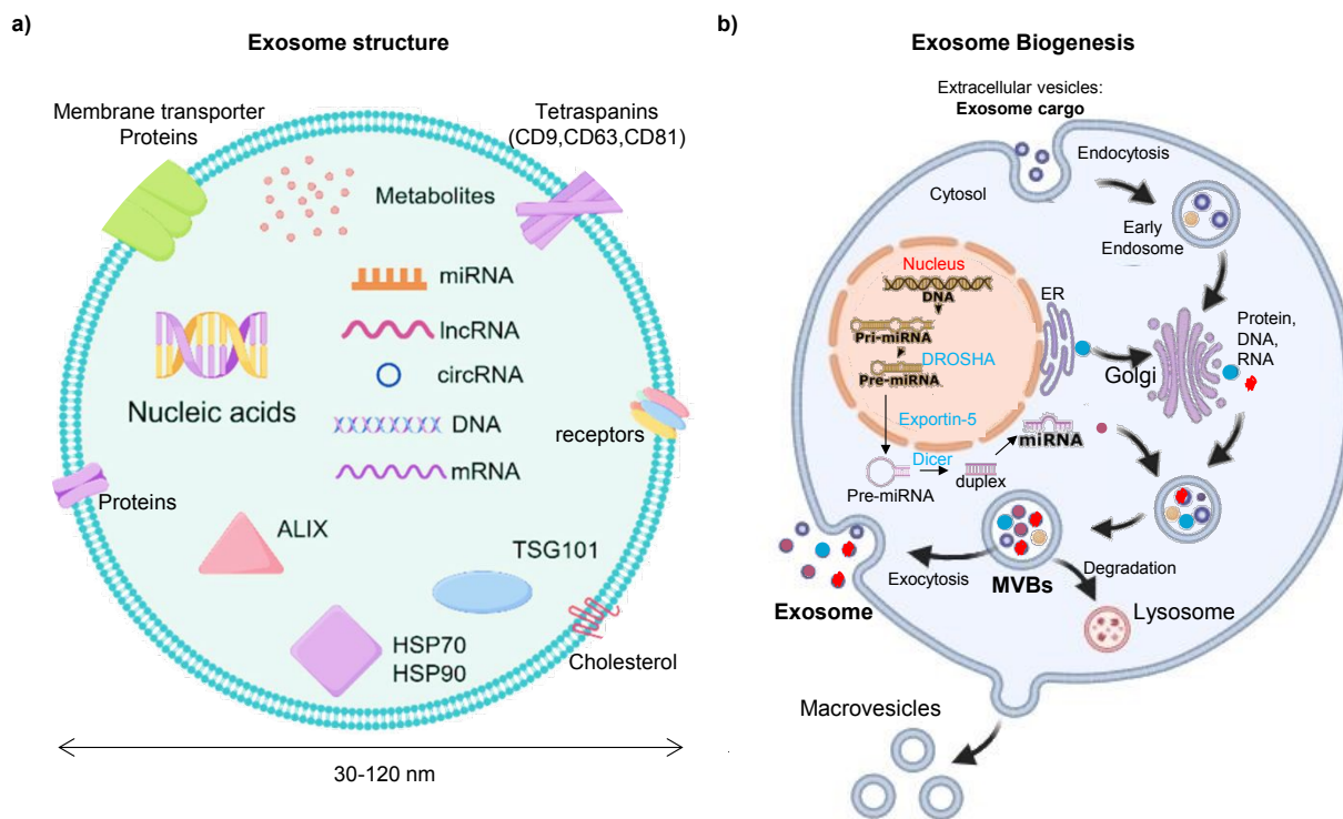
Figure 2: Exosome structure and biosynthesis. A) Exosome size and functional components such as miRNA, mRNA, circRNA, proteins, and lipids. 48 B) miRNA is transcribed in the nucleus, processed by Drosha and Dicer, and loaded into RISC. Exosomes are released from MVBs and carry miRNA to recipient cells. 40
