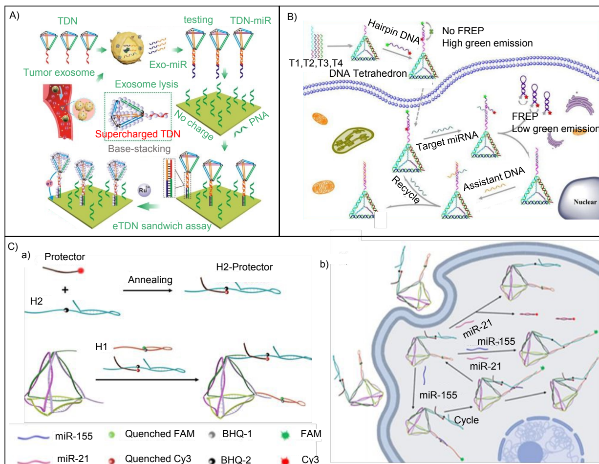
Figure 4. (A) Illustrative diagram of TDNs synthesis for nanolabel supercharge-based electrochemical platform for exo-miR analysis, 149 (B) the diagrammatic representation of the designed DTNP-based FRET detecting sensor for miRNA analysis in living cells, 142 (C) synthesis of FDTp sensors for two types of miR-21 and miR-155 imaging in living cells. 154
