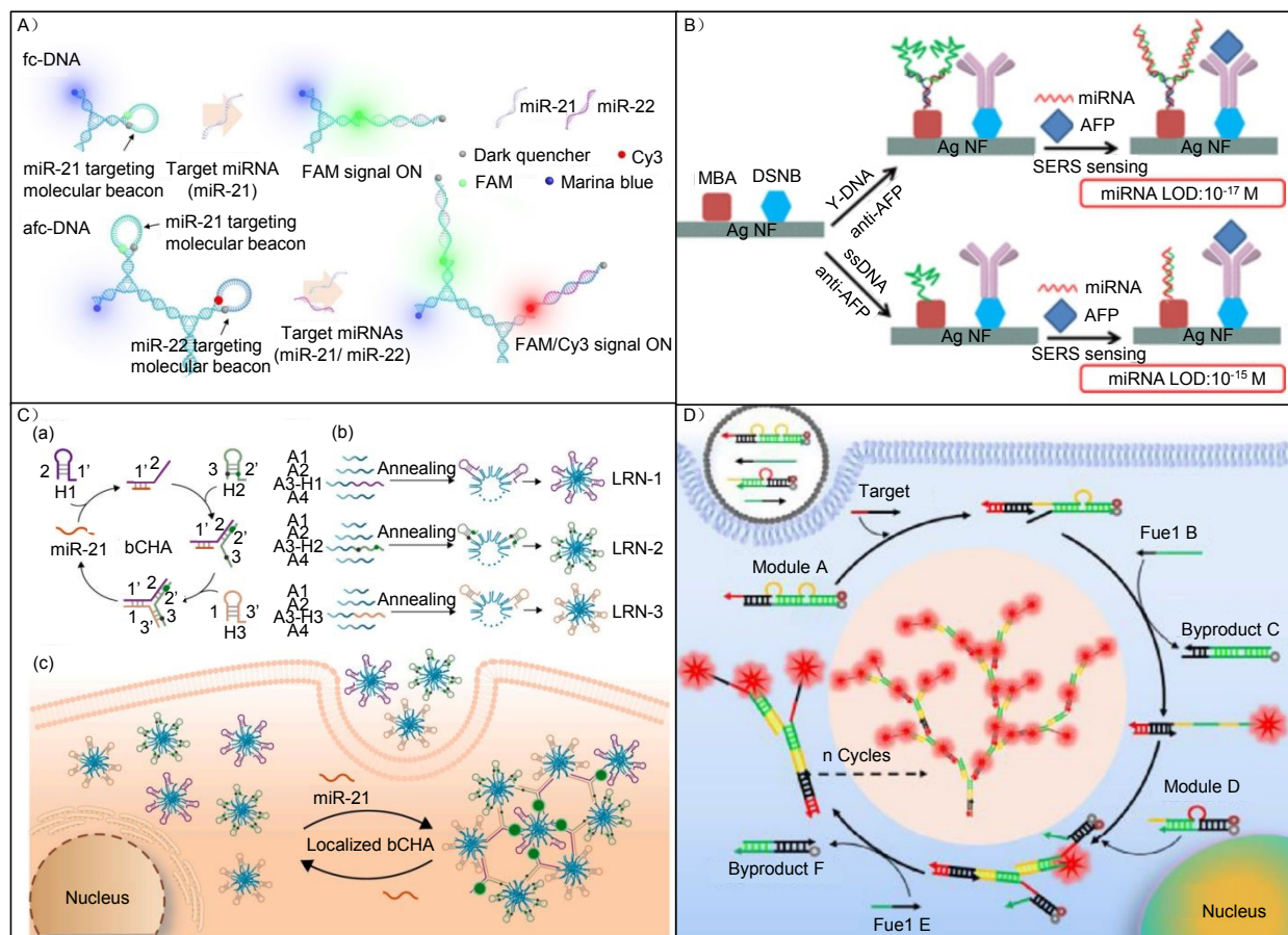
Figure 5. (A) Branched DNA nanomaterials with fluorescent dyes for intracellular miR-22 and miR-21 detection, 161 (B) branched DNA-based AgNF for detecting AFP and miRNA on SERS, 166 (C) synthesis of branched DNA nanomaterials for miR-21 detection in living cell, 168 (D) schematic diagram of a 1:L platform by target triggered synthesis of DNA dendrimers for contrast-increased imaging of miRNA in living cells. 169
