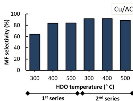
Fig. 10 MF selectivity in furanics obtained from molten salt hydro-pyrolysis of pinewood and subsequent hydrodeoxygenation with Cu/AC, displayed by the experimental series. Conditions: 0.4 MPa and hydro-pyrolysis at 350 °C.
