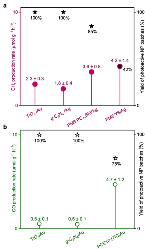
Fig. 2 (a) \text{CH}_4 production rates in \text{CO}_2 reduction reactions with PM6:PC 71 BM/Ag and PM6:Y6/Ag NPs. (b) \text{CO} production rate in \text{CO}_2 reduction reactions with PCE10:ITIC/Au NPs. The results are compared to the rates obtained under identical conditions with the benchmark photocatalysts \text{TiO}_2 (P25) and g\text{-C}_3\text{N}_4 , functionalised with Ag or Au cocatalysts. The yield of photoactive NP batches indicates the reproducibility of the production rates across 8 or 10 reactions.
